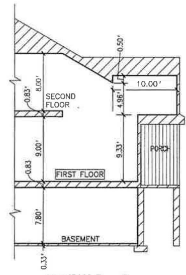
SECTION D - D
