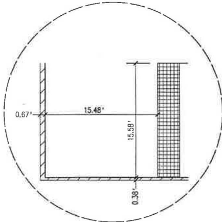
ALTERNATE FLOOR PLAN
