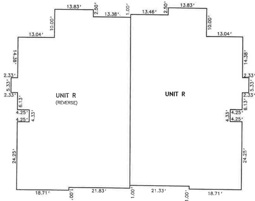
PERIMETER PLAN FOR BUILDING 30
